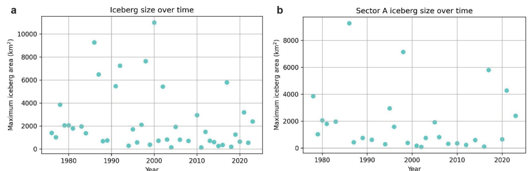
Figure 2. Annual maximum calving events for (a) all of Antarctica and (b) Sector A between 1976 and 2023.
